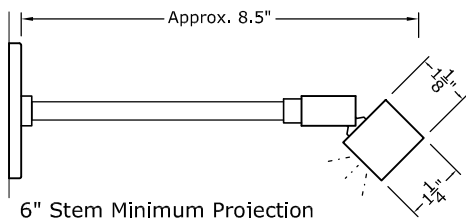
6" Stem Minimum Projection (Specify Stem 6", 10", 16" or Custom Stem w/ Length Between 6"- 16")
