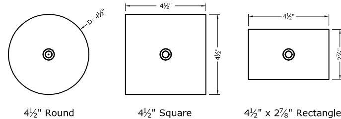
Mounting Plate Options (MM01B Screwless):
