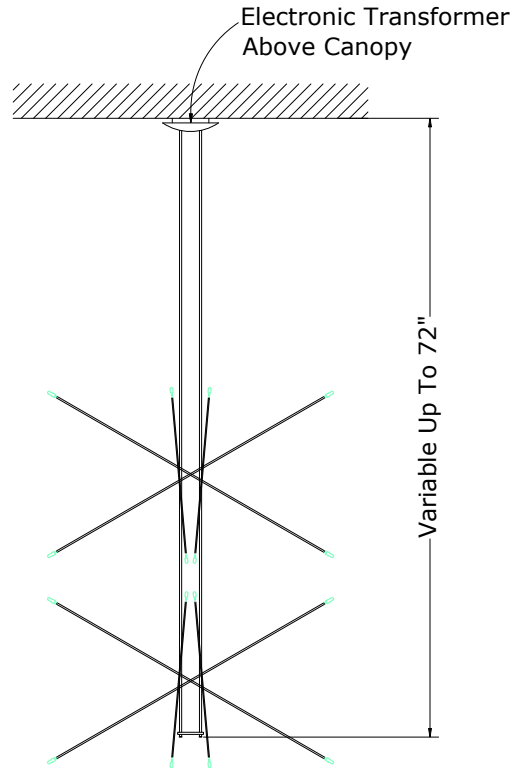
Side View 2 Tiers (4 Arm Per Layer)
