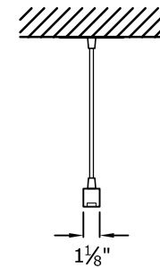
Side View 10" Drop Minimum, Greater Drop Preferred
