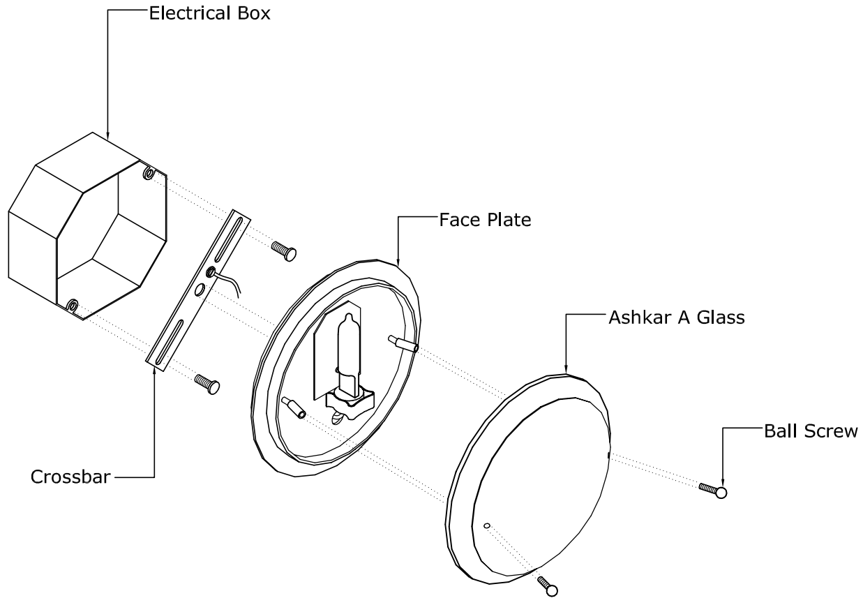
Assembly For Round and Square Face Plates
