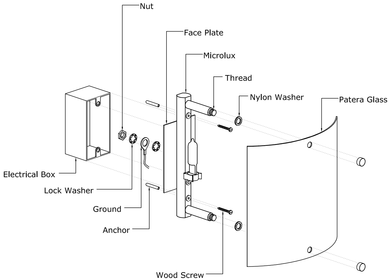
Axonometric View
